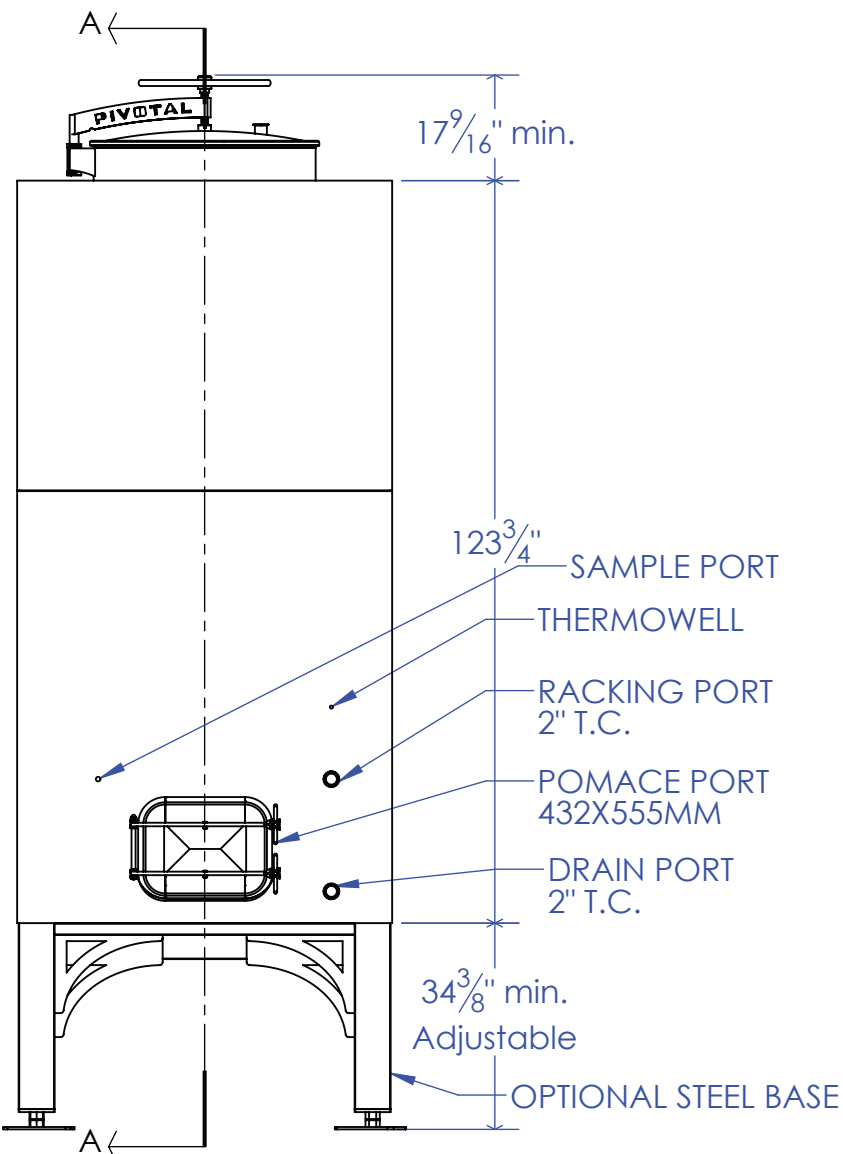
FRONT
